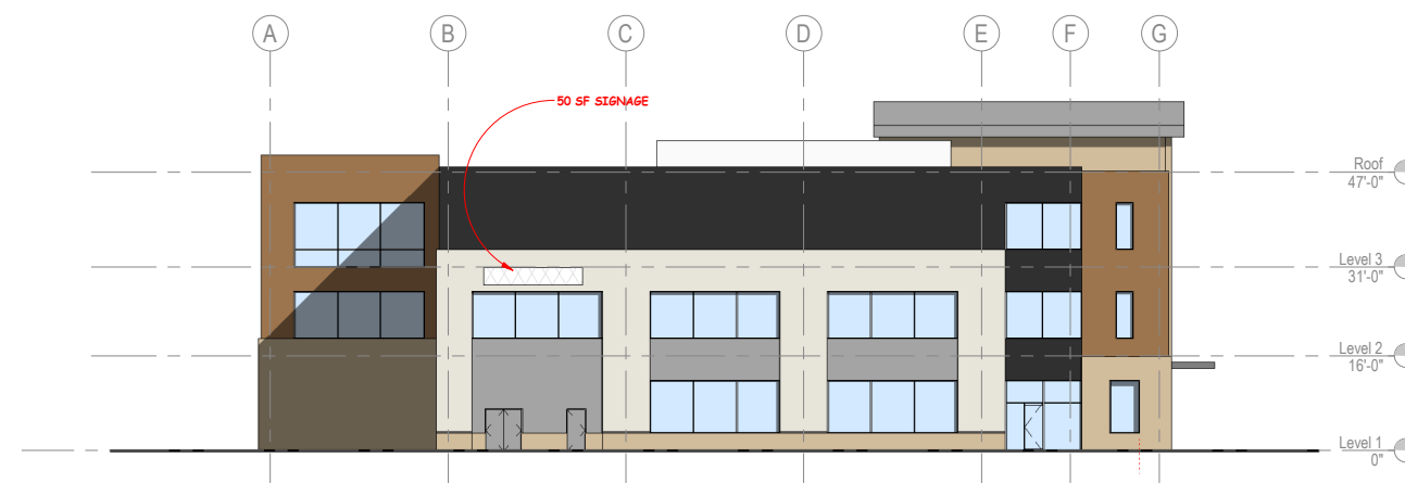
WEST ELEVATION - LLYOD
